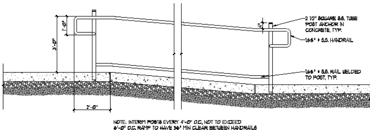
SECTION - HANDRAIL AT RAMP
